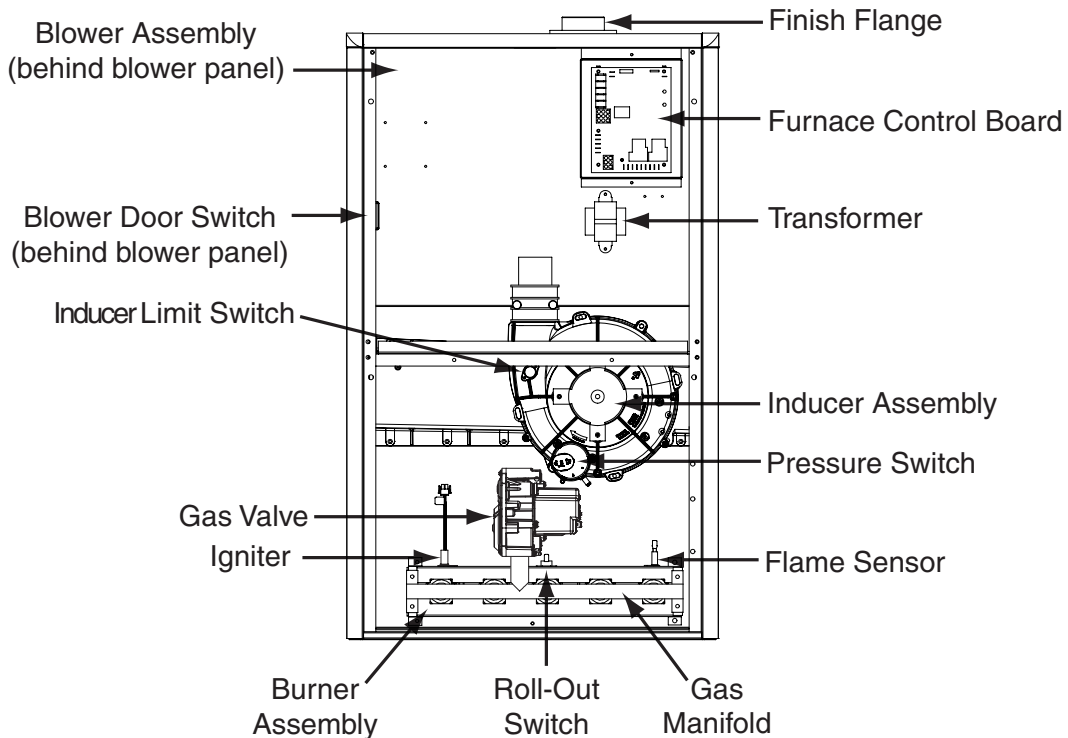
Downflow Furnace
