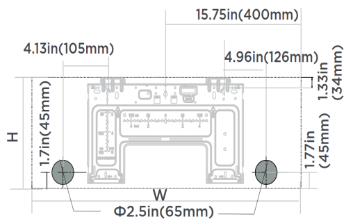
Indoor unit dimensions(WxH): 28.7in(729mm)x11.5in(293mm)
