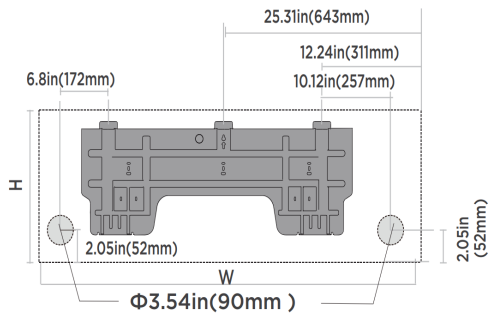
Indoor unit dimensions(WxH): 49.57in(1259mm)x14.25in(362mm)
