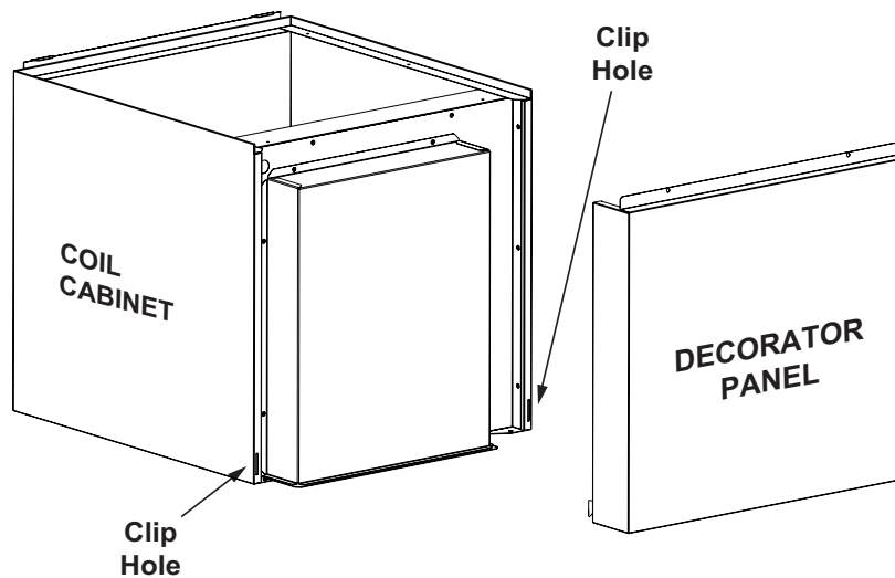
Figure 2. Coil Cabinet with Decorator Panel
