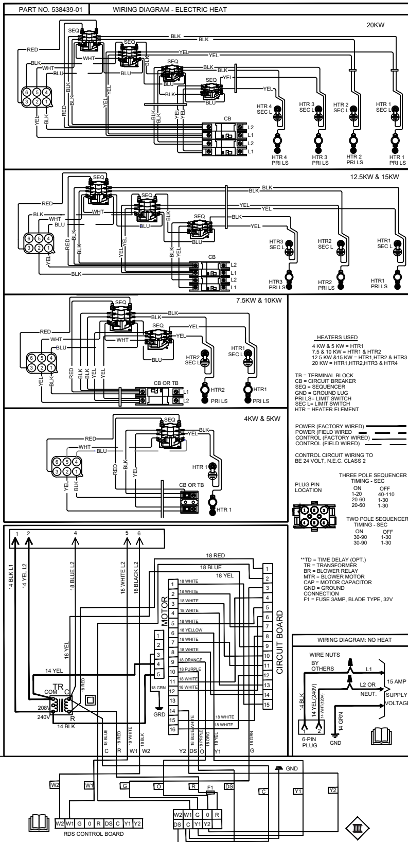
FIGURE 13. Air Handler with Electric Heat – Variable-Speed Motor – RDS Controller
