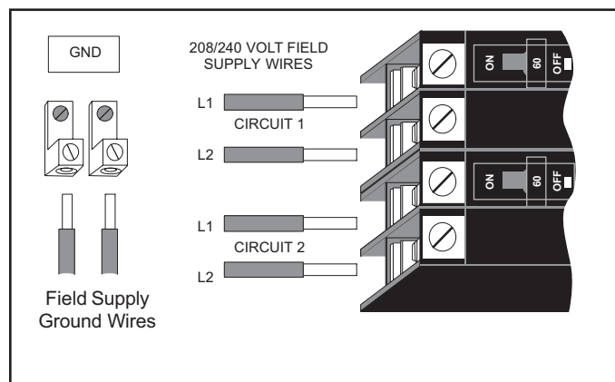
FIGURE 5. Field Power Supply Wiring
