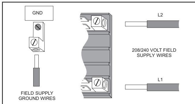
FIGURE 6. Terminal Block Connections
