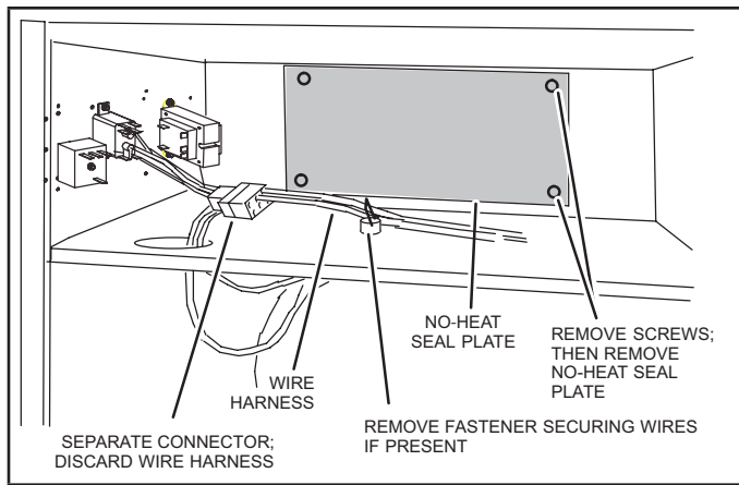
FIGURE 1. Prepare to Install Heat Element
