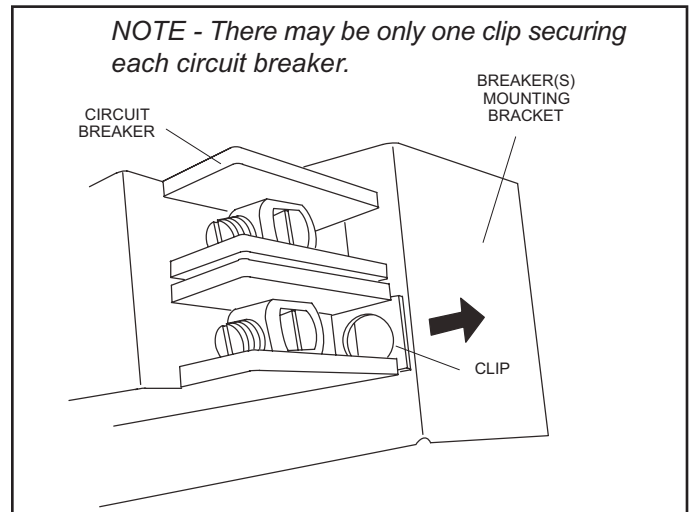
FIGURE 3. Circuit Breaker Clip
