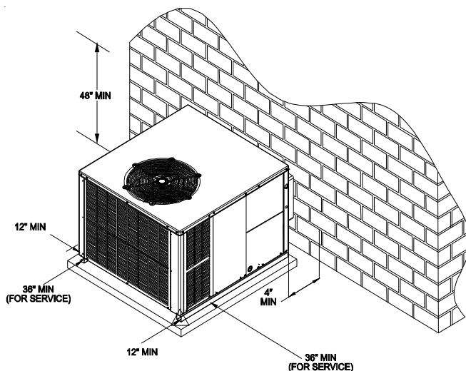
Outside Slab Installation -Multi-positional (M)
