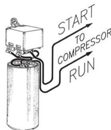
CSIR COMPRESSOR
