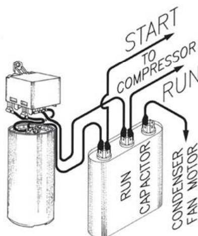
DUAL CAPACITOR
