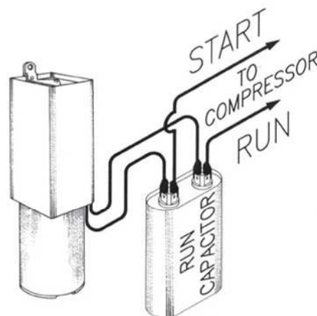
STANDARD CONNECTION
