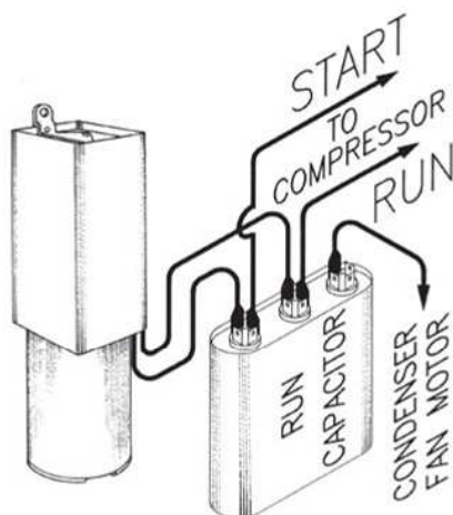
DUAL CAPACITOR
