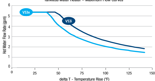
Tankless Water Heater – Maximum Flow Curves
