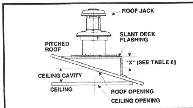
Figure 17. Example of Flat Jack with Flashing
