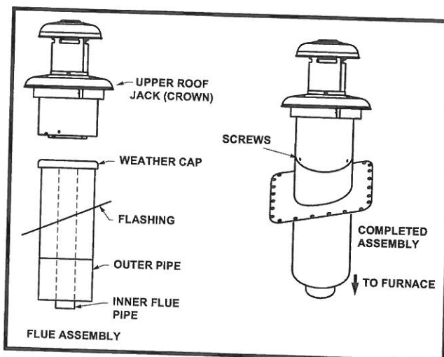
Figure 23. Roof Jack Crown
