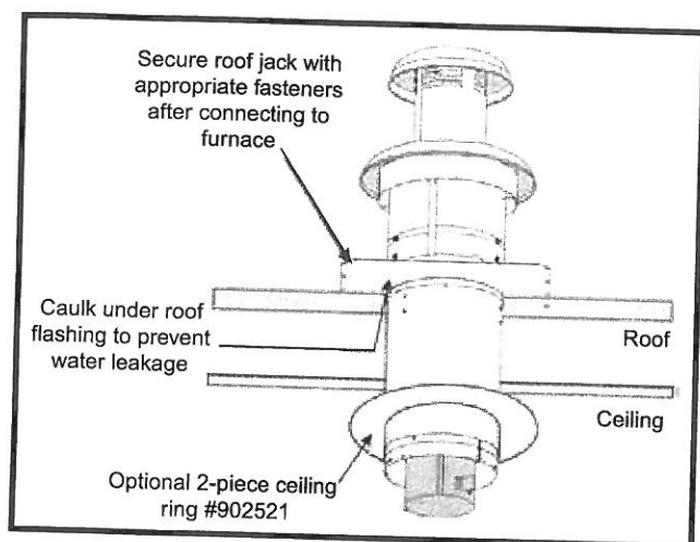
Figure 20. Flat Roof
