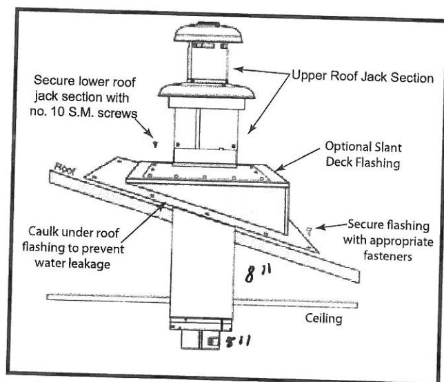
Figure 21. Pitched Roof
