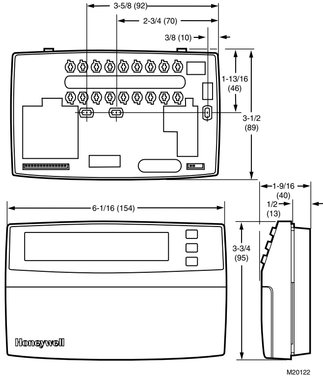
Fig. 1. T8665A dimensions in in. (mm).
