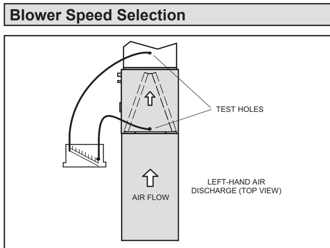
FIGURE 9. Static Pressure Test
