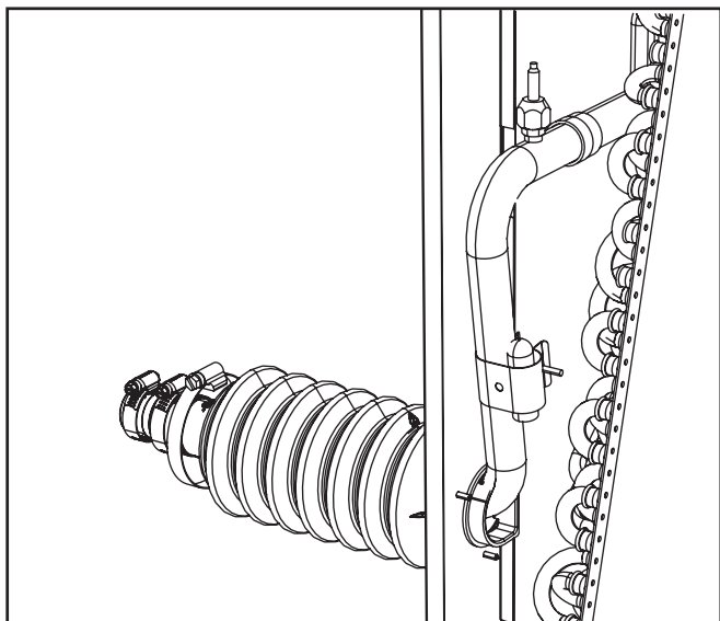
FIGURE 4. BC7*C-71 Suction Line with Line Set Joint Sleeve
