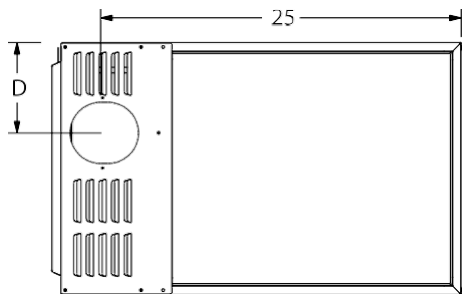
Upflow /Horizontal
