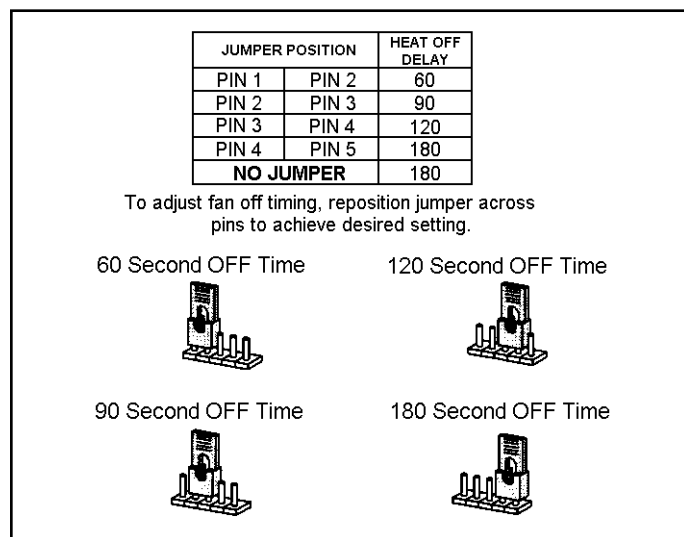
Figure 35. Heat Fan Off Time in Seconds
