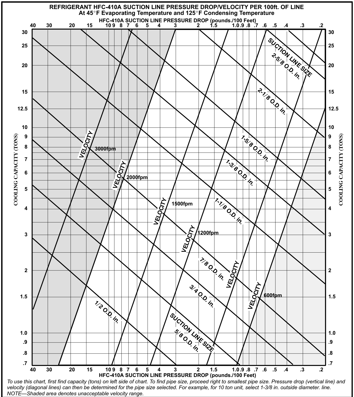
Figure 7. HFC-410A Suction Line
