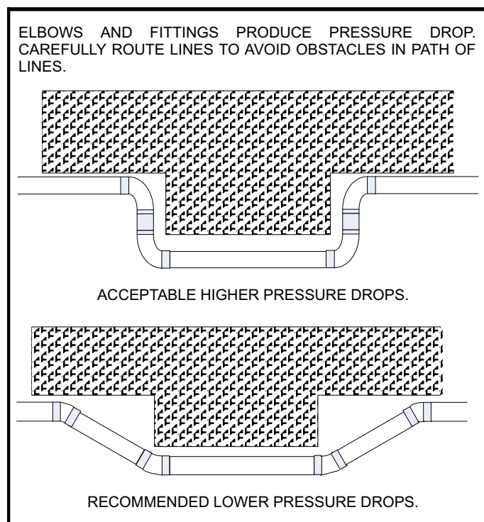
Figure 3. Pressure Drops
