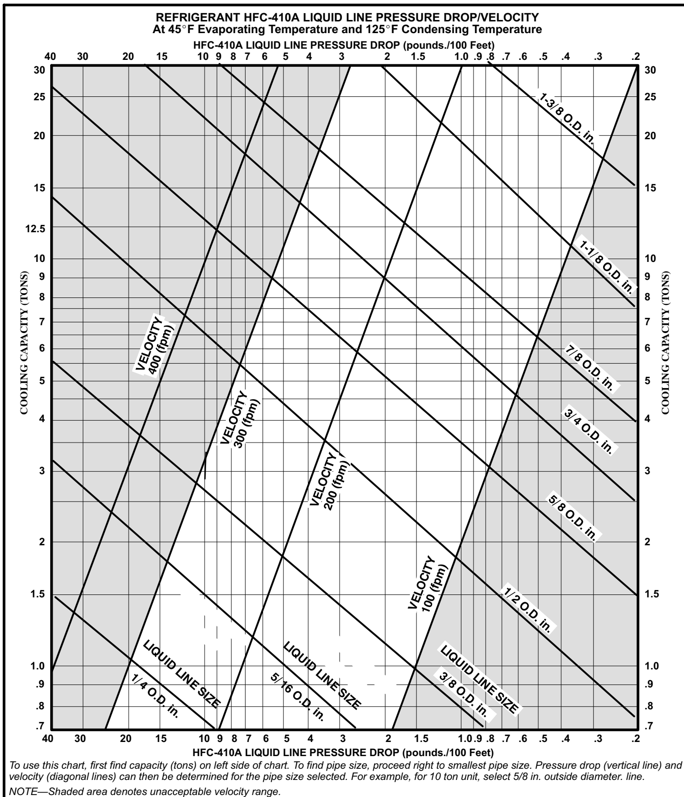
Figure 5. HFC-410A Liquid Line
