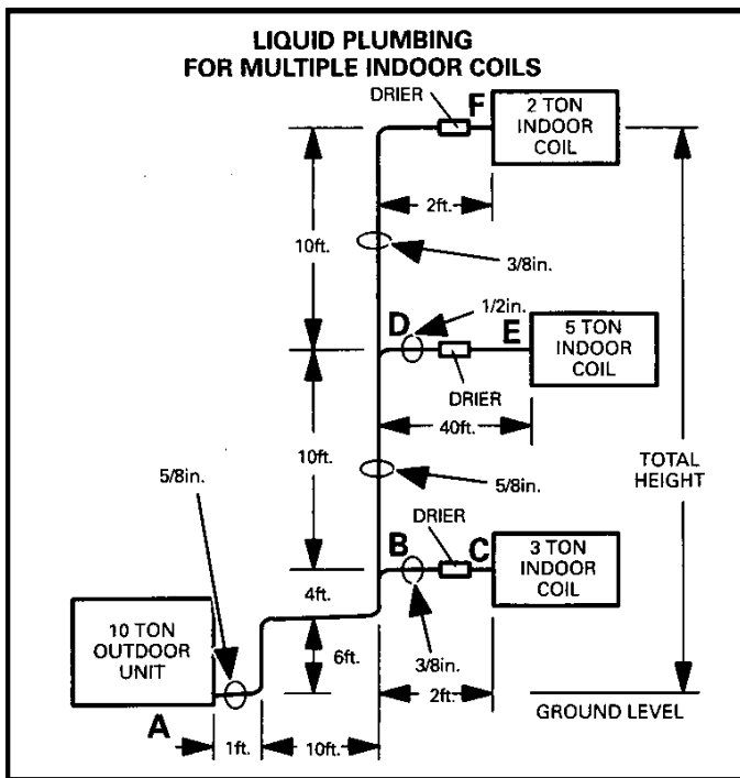
Figure 22. Liquid Plumbing
