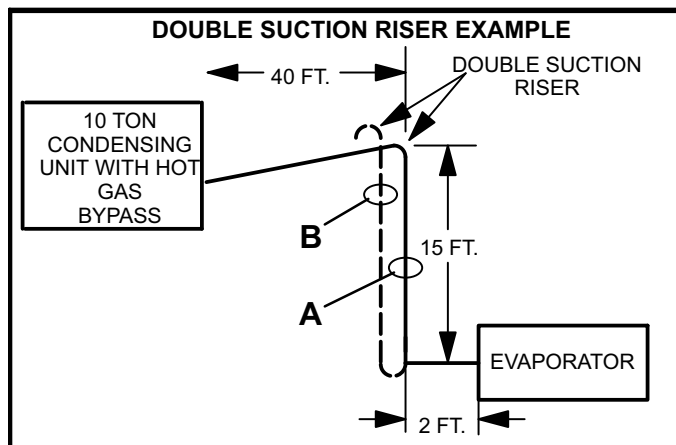
Figure 16. Double Suction Riser
