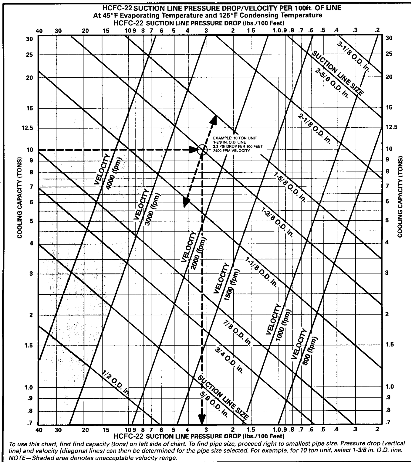
Figure 6. HCFC-22 Suction Line
