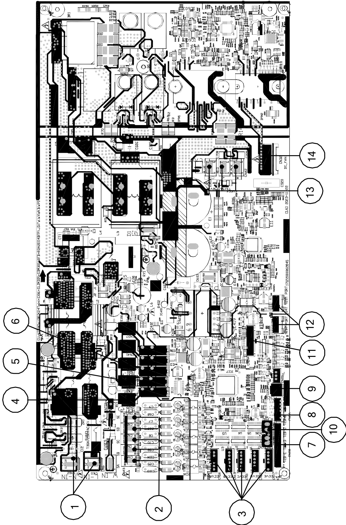
Outdoor unit printed circuit board diagram: 1712200062845
