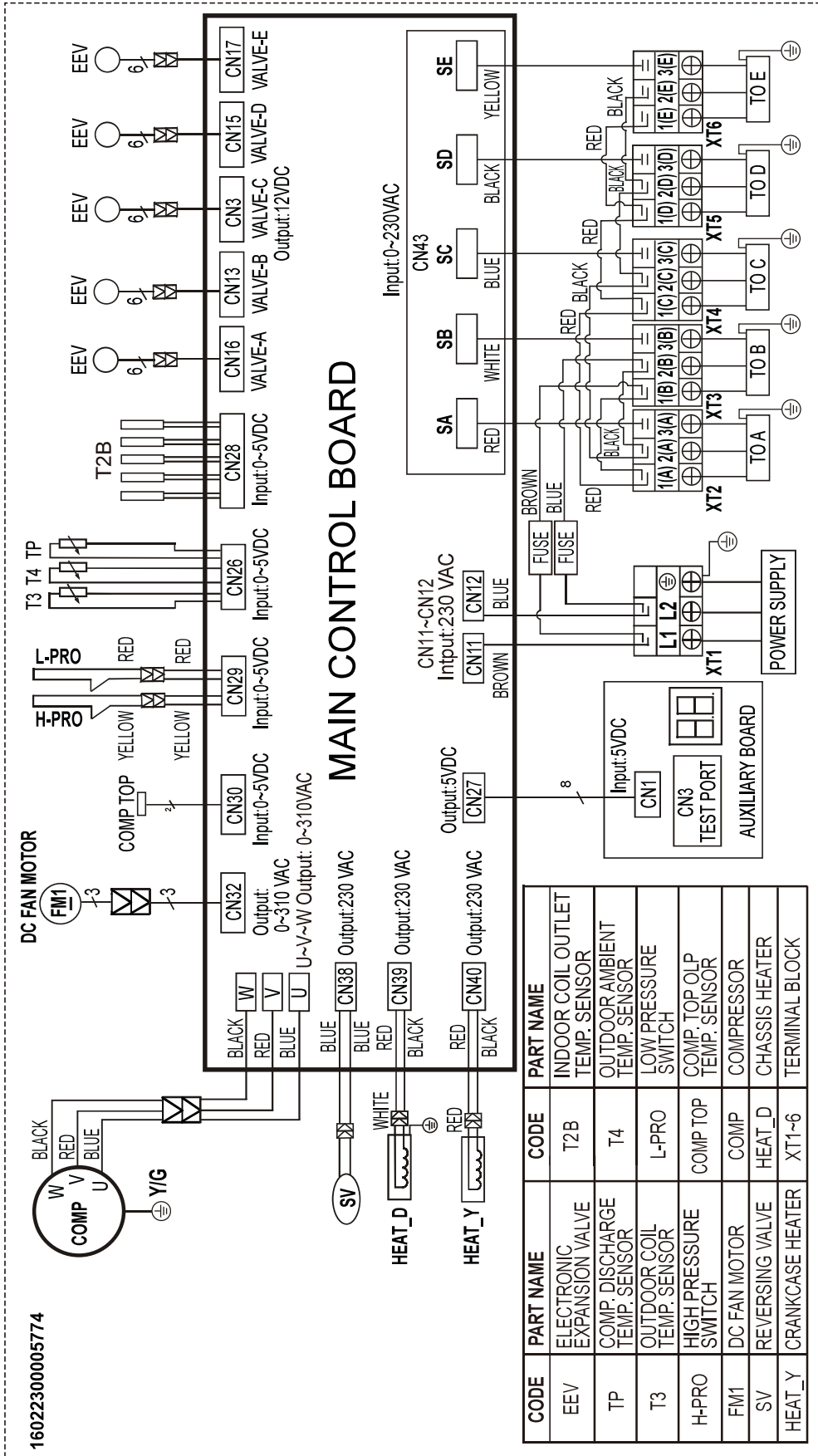
Outdoor unit wiring diagram:16022300005774
