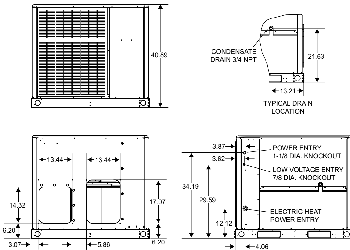
SIDE VIEWS
