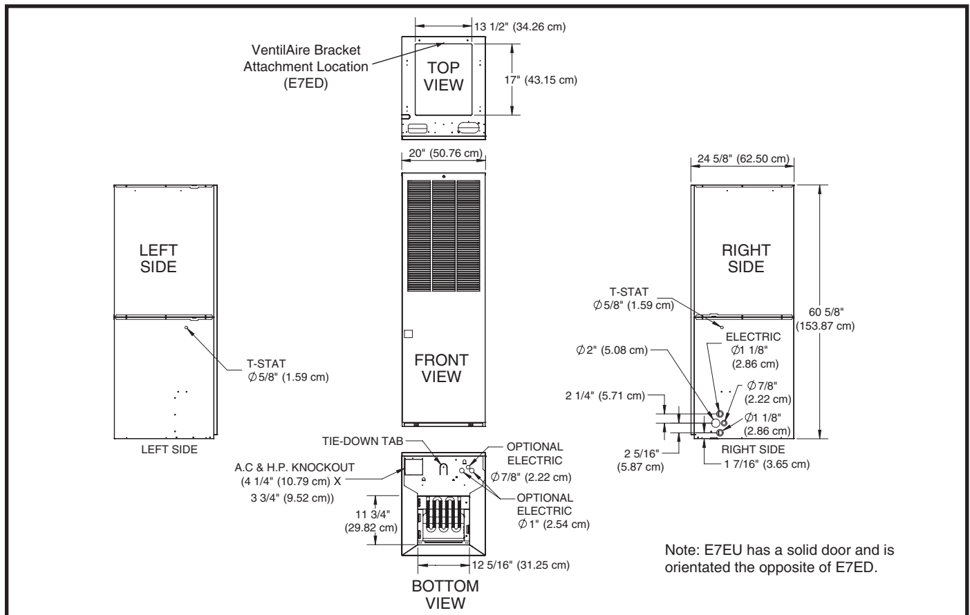
E7ED Physical Dimensions
