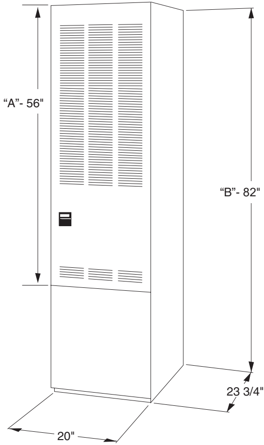
"A" Model without Coil Cabinet "B" with optional 26 in. Coil Cabinet (not included)
