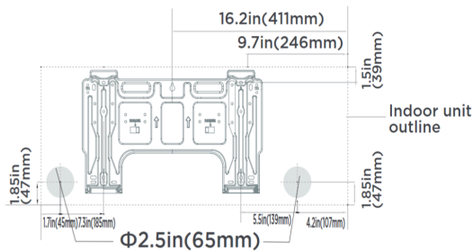
Indoor unit dimensions: 31.7in(805mm)x11.2in(285mm)
