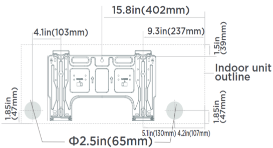
Indoor unit dimensions: 28in(715mm)x11.2in(285mm)
