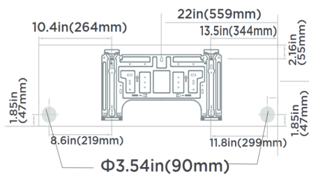
Indoor unit outline
